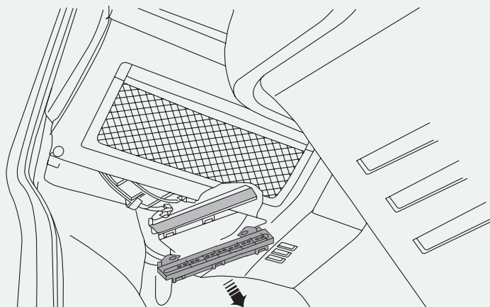
STEP 4 Pull filter cover down and out to remove, pull used filter out from housing.
