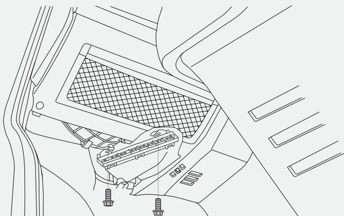
STEP 3 Remove 2 hex headed screws as shown.
