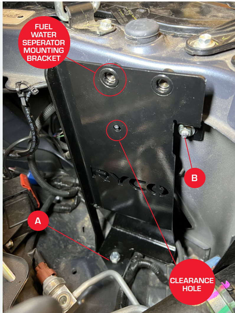
FIGURE 1A FUEL WATER SEPERATOR MOUNTING BRACKET INSTALLATION
